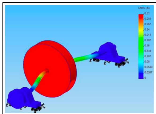
Figure 12. Estimation of the assumed modeled frequency by the Finite Element Method. Result: \omega_m \simeq 44 Hz.
