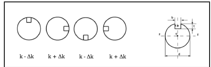
Figure 16. Variable stiffness of the rotor induced by the slot along its length. Conditions: b=5 mm, t=2.65 mm, d=15 mm. I_z = 2485 - 331.25 \cdot 10^{-12} \text{ m}^4 .
