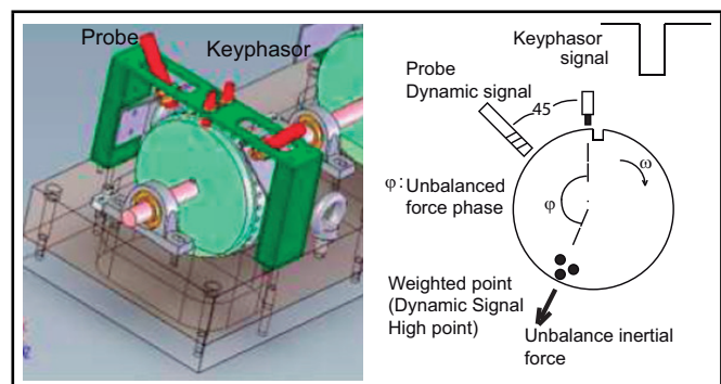
Figure 3. Analog Probe plus digital Keyphasor layout at the measurement bridge.
